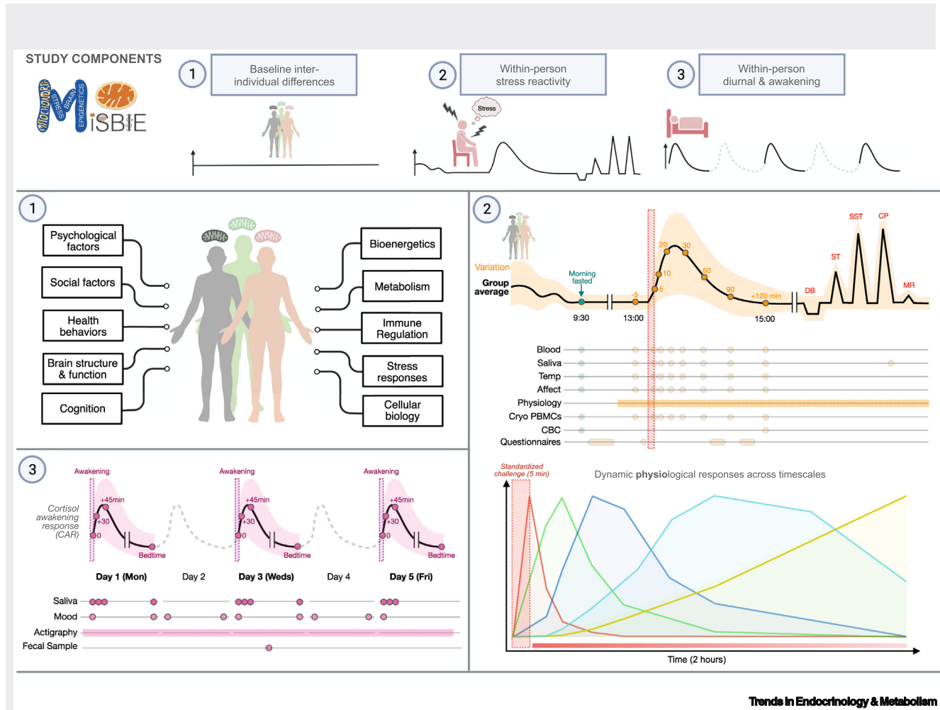
Figure 1. MiSBIE study components. MiSBIE assesses all hallmarks and principles of human psychobiology. (top) The three major MiSBIE components include (1) highly controlled laboratory-based baseline measures of biomarkers, mitochondrial biology, and other outcomes, (2) a validated experimental speech delivery stress reactivity paradigm, and (3) home-based data and sample collection. ① Baseline measures capture stable traits of individuals along the spectrum of normal and abnormal OxPhos capacity, reflecting the stable state of the organism. ② Stress-reactivity and recovery measures capture the robustness, resilience, and adaptability of the organism to psychosocial stress, deep breathing (DB), standing transition (ST), 30-second sit-to-stand test (SST), and cold pressor (CP), and metabolic rate measurement (MR). Different biomarkers exhibit distinct expected kinetics from which indices of reactivity, recovery, resilience, and elasticity can be computed. ③ Home-based data collection captures daily cycles of sleep and awakening in biological, psychosocial, and behavioral outcomes from four saliva samples per day, two sets of mood-related questionnaires (AM, evening), and continuous wrist actigraphy. Abbreviations: CBC, complete blood count; PBMCs, peripheral blood mononuclear cells.
