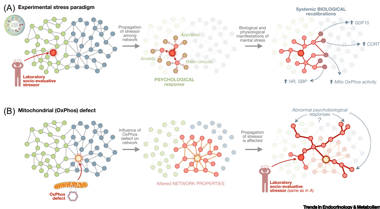
Figure 2. Model of mind–body processes emerging from information flow across the psychobiological network. (A) An experimental paradigm where a standardized laboratory psychosocial stressor [e.g., Trier Social Stress Test (TSST) speech task] triggers proximal psychological processes that ripple out into diverse brain–body systems functionally interconnected and regulated by mitochondrial oxidative phosphorylation (OxPhos). Pre-existing disturbances (e.g., hunger), disorders (e.g., anxiety), and symptoms (e.g., pain) affecting specific nodes of the psychobiological network not illustrated here also could influence both the perception of the stressor and the nature and magnitude of the response elicited by the stressor. (B) Study design where the mitochondrial OxPhos node is perturbed, as in primary mitochondrial diseases. This leads to cellular and physiological recalibrations that influence how the same stressor as in (A) can produce distinct (exaggerated, blunted, or qualitatively distinct) psychobiological responses. The 2D psychobiological network is a static simplification of the complex dynamical system that is the human organism. Abbreviations: CORT, cortisol; GDF15, growth differentiation factor 15; HR, heart rate; SBP, systolic blood pressure.
